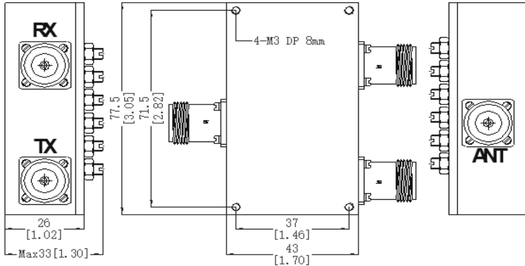
Physical Dimensions ( \pm 0.3\text{mm} )
