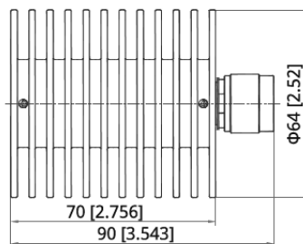
TER-N50M-985002 Dimensions
