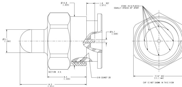
TER-N50M-985002 Dimensions
